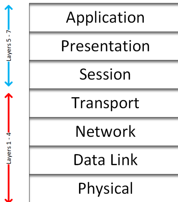
OSI Model
