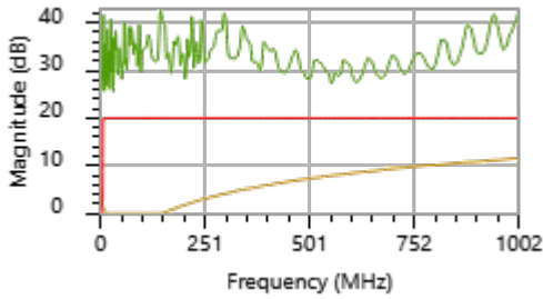
Return Loss
